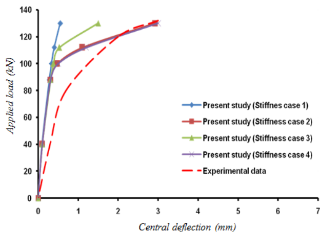
Fig. 10. Load-deflection curve for SFRC beam 1 with c=25\text{mm} .
