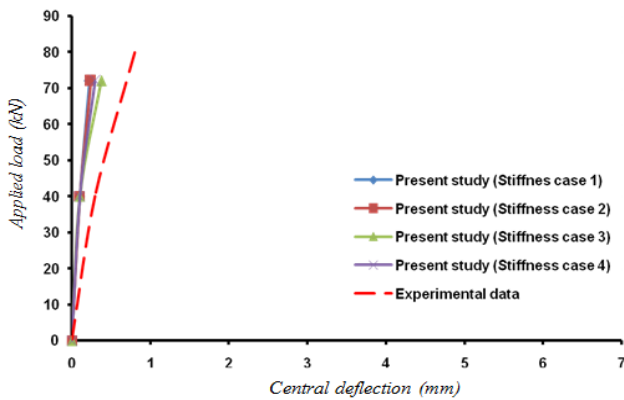
Fig. 9. Load-deflection relationship for SFRC beam 1 with c=15\text{mm} .
