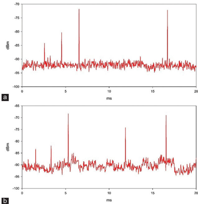
Fig. 22. Zero span of partial discharge detection in N_2O_2Ar gas at 1.42 GHz using (a) PDU-G2 external antenna and (b) proposed log-periodic dipole array antenna.
